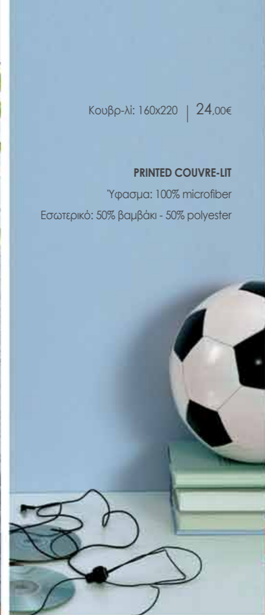
join - blue
